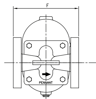
INTEGRAL FLANGE
